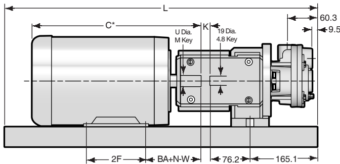
T31 SERIES WITH P2 BEARING FRAME
